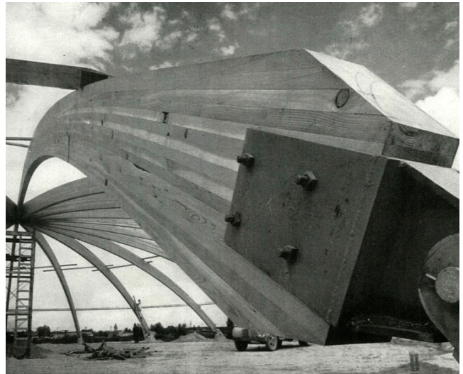
Arches for the Hunt School cafeteria-auditorium in Tacoma, Washington, designed by Robert B. Price.
